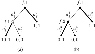
Figure 2: Game that we use to prove that perturbed SSEs and WSEs are not refinements of SSEs and WSEs.
